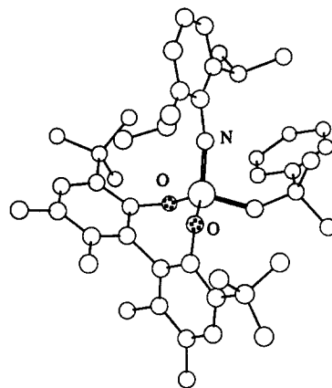
Figure 3. X-ray structure of complex 1a .
