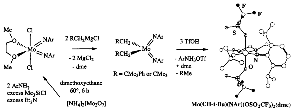
Scheme 1. Synthesis of \text{Mo}(\text{CHCMe}_2\text{Ph})(\text{NAr})(\text{triflate})_2(\text{dme}) .
