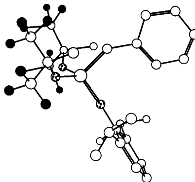
Figure 1. The X-Ray Structure of \text{W}(\text{CHPh})(\text{NAr})[\text{OCMe}(\text{CF}_3)_2]_2 .
