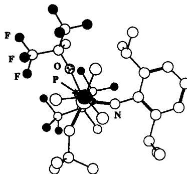
Figure 2. X-ray Structure of Mo(CHCMe_3)(NAr[OCMe(CF_3)_2]_2)(PMe_3) .
