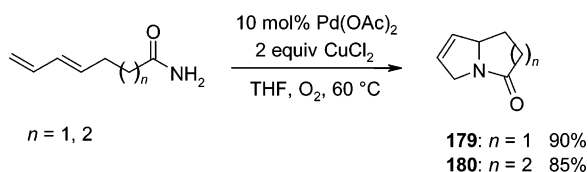
Scheme 136
