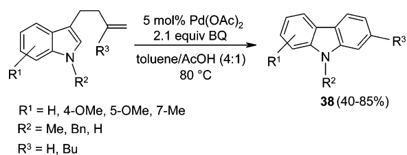
Scheme 33
