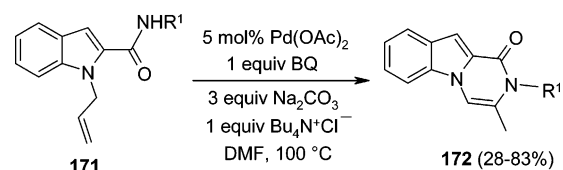
Scheme 130
