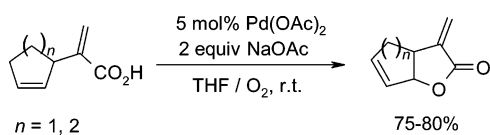
Scheme 89
