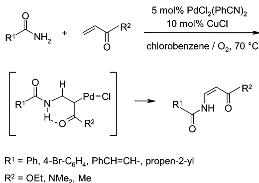
Scheme 141
