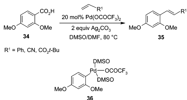
Scheme 29
