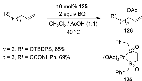
Scheme 102
