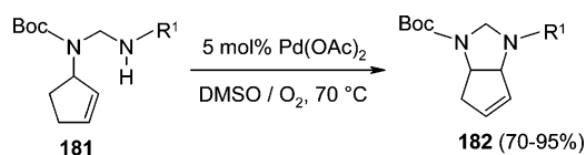
Scheme 136
