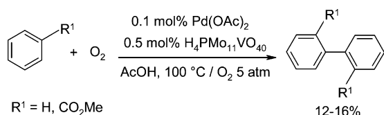
Scheme 45
