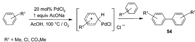
Scheme 45
