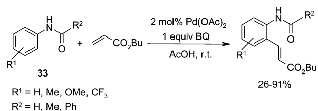
Scheme 28
